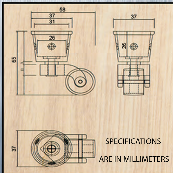
ROUND CASTERS
