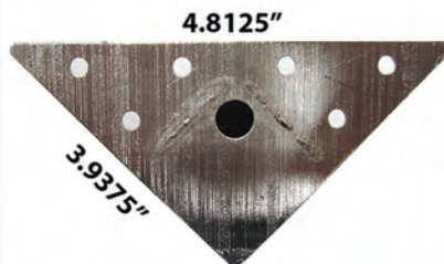
TOP PLATE
