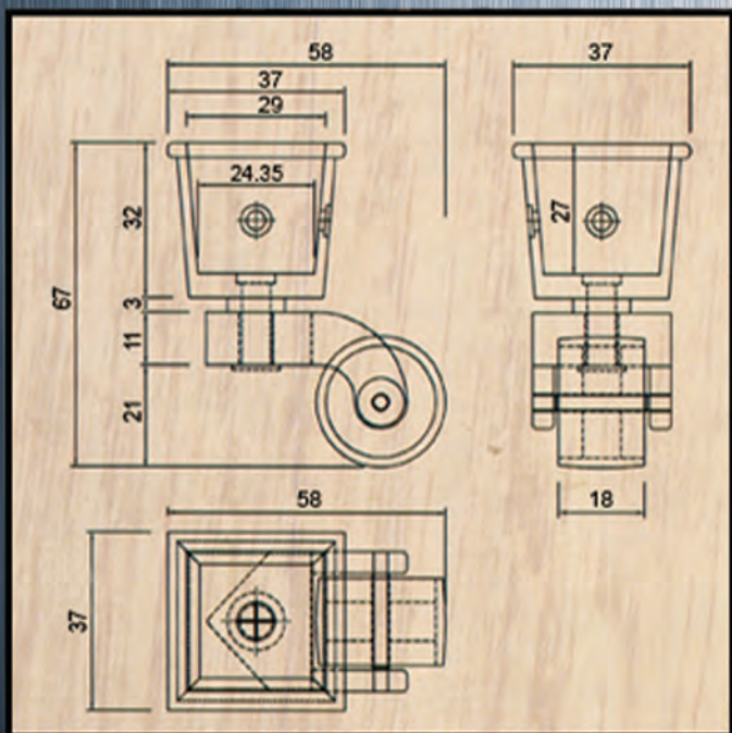
SQUARE CASTERS
